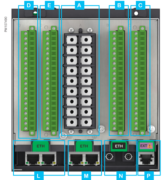
PowerLogic P5x30 - CT/VT variant
