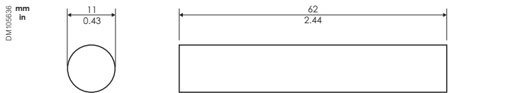
Arc-flash sensor: Pipe type
