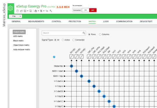
Output matrix view of eSetup Easergy Pro
