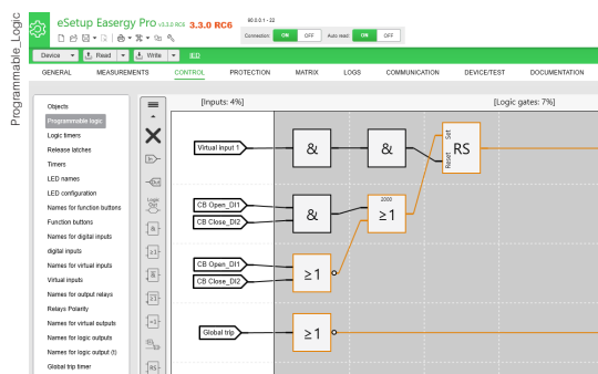
Programmable logic view of eSetup Easergy Pro
